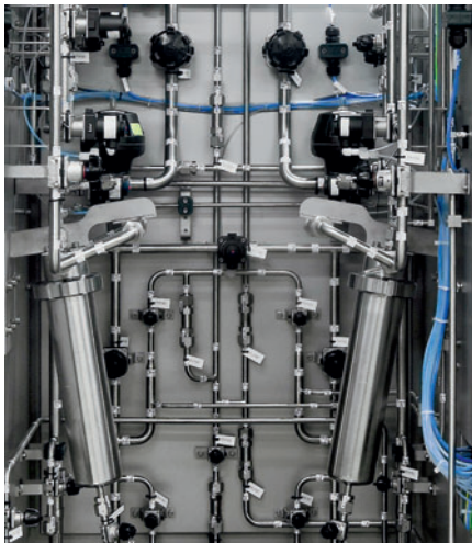
Stainless steel components with plastic actuators
